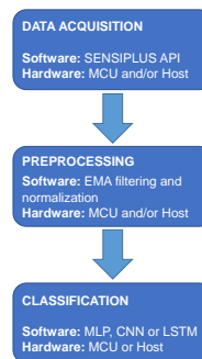
Figure 2: The proposed integrated system. SDM stands for SENSIPLUS Deep Machine.
