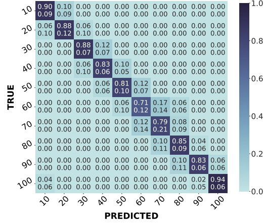
Figure 9: Obtained confusion matrix of the Support Vector Machine model, with mean value (top) and standard deviation (bottom) for each class.
