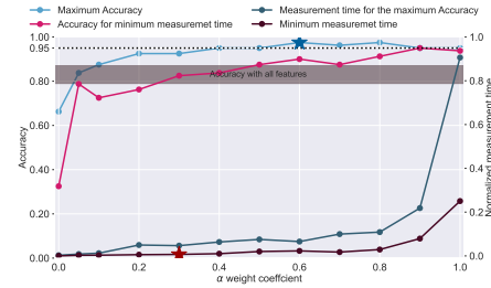
Figure 10: Accuracy and measurement time as a function of \alpha weight coefficient for PSO+SVM combination.
